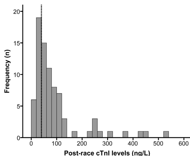
Fig. 1. Frequency distribution of cardiac troponin I levels (cTnI) in 82 athletes directly after the finish of the Eindhoven marathon. The average cTnI level increased from 14 \pm 12 ng/L at baseline to 94 \pm 102 ng/L directly post-exercise. In addition 55 (69%) of our participants exceeded the clinical cut-off value for an acute myocardial infarction (represented by the dashed line).
